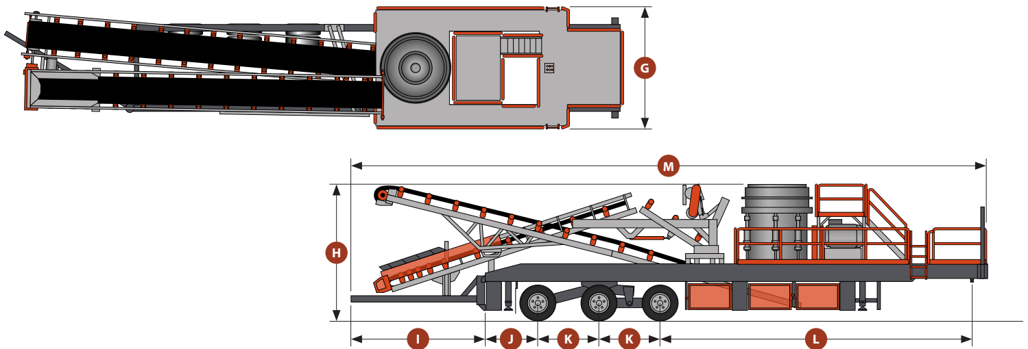
TRAVEL DIMENSIONS - INCHES (MM)
